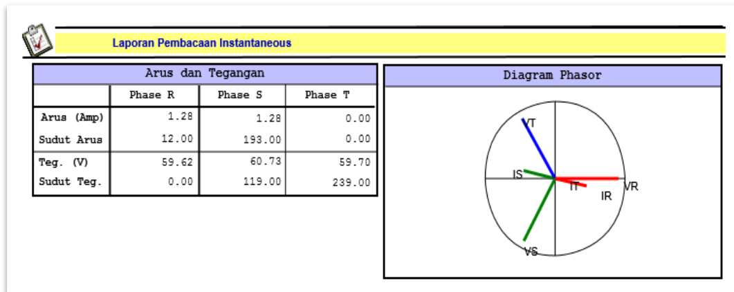
Gambar 2.16 Phasor CT Rusak
