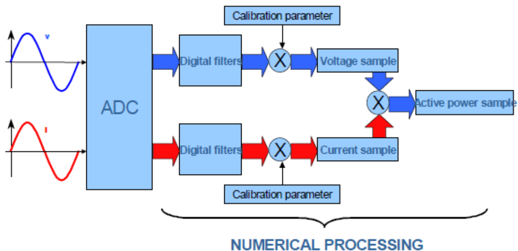
Gambar 2.3 Proses Analog Digital Converter
