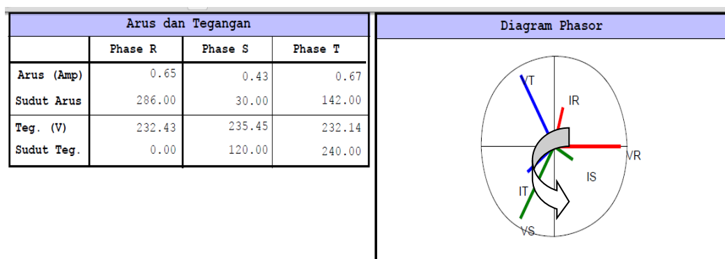
Gambar 2.12 Phasor Beban Kapasitif
