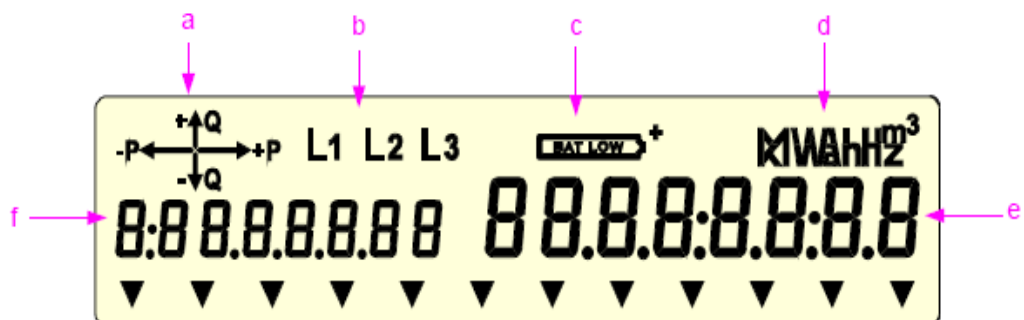
Gambar 2.5 Tampilan LCD
